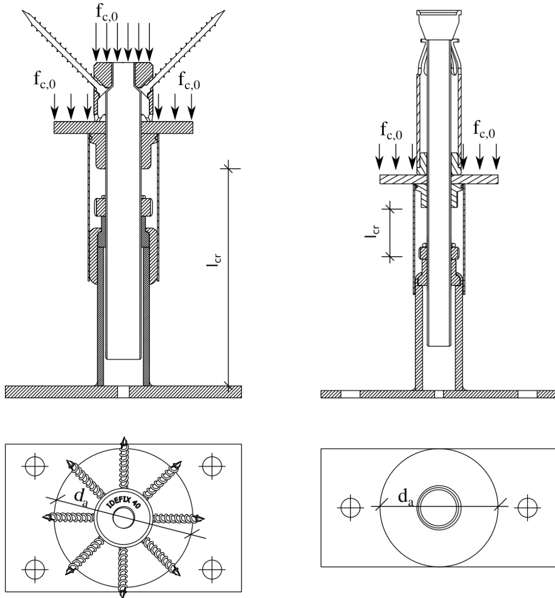
Figure 23: post bases IdeFix STF and ZaFix STZ 300, 400,700, buckling length and compressive stresses
