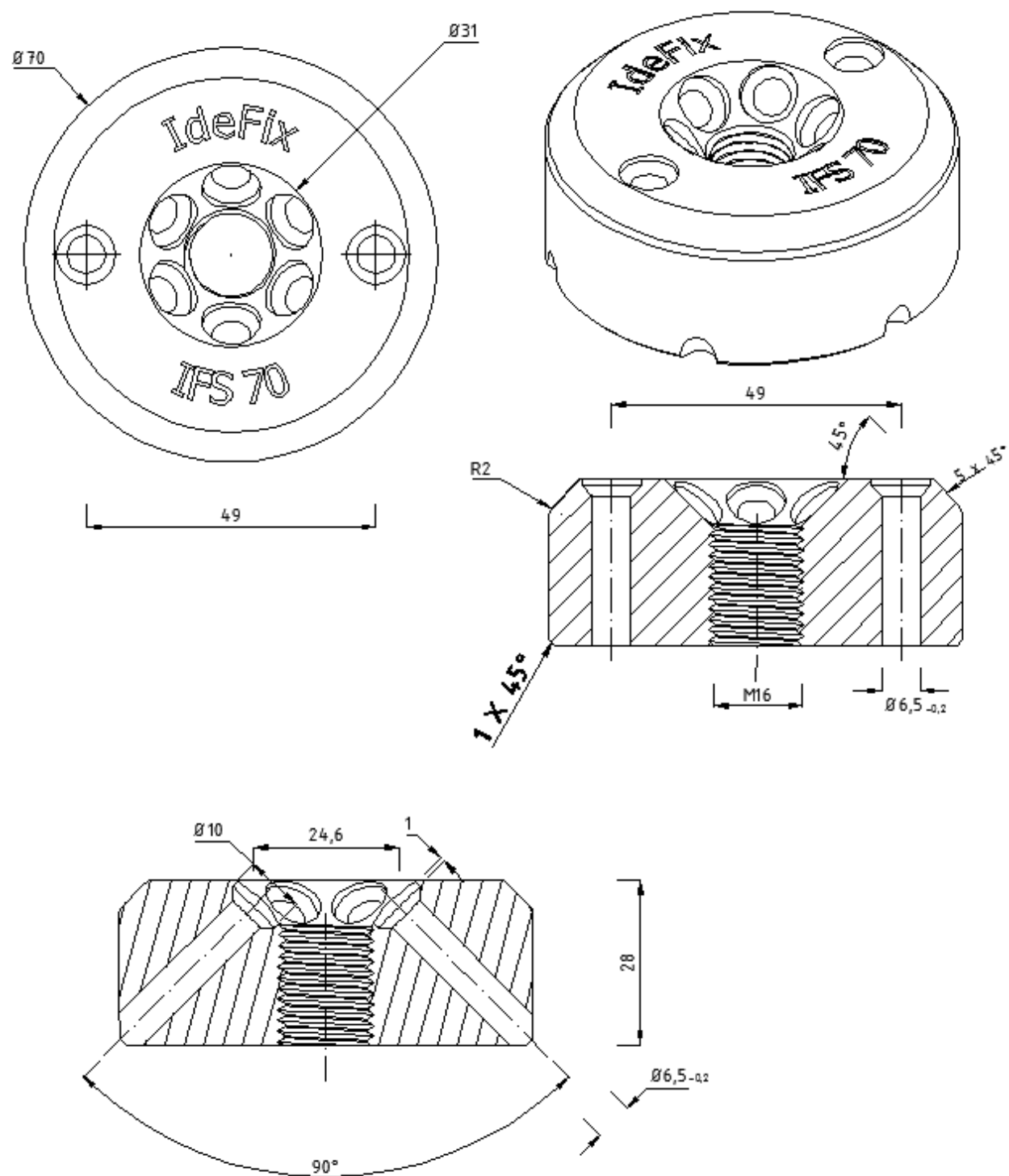
Figure 17: IdeFix IFS, details
