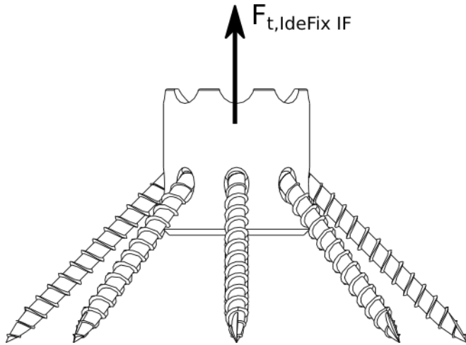
Figure 1: IdeFix IF in tension loading
